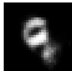
FC-AE
